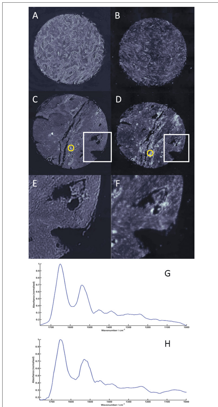
Figure 1. Spectral images of the 1650\text{cm}^{-1} band intensity across medullablastoma (A and B) and glioblastoma (C, D, E and F) tissue cores (approximately 1.5\text{mm} diameter and 5\mu\text{m} thickness) imaged using a Spero QCL microscope (A, C and E) and a 128 \times 128 FPA microscope system (B, D and F). 1E and 1F are zoomed images of the areas highlighted by the white boxes in 1C and 1D of the glioblastoma tissue core. Spectra from the areas highlighted in yellow on C and D are shown for the QCL microscope (G) and for the FT-IR microscope 128 \times 128 system (H).
