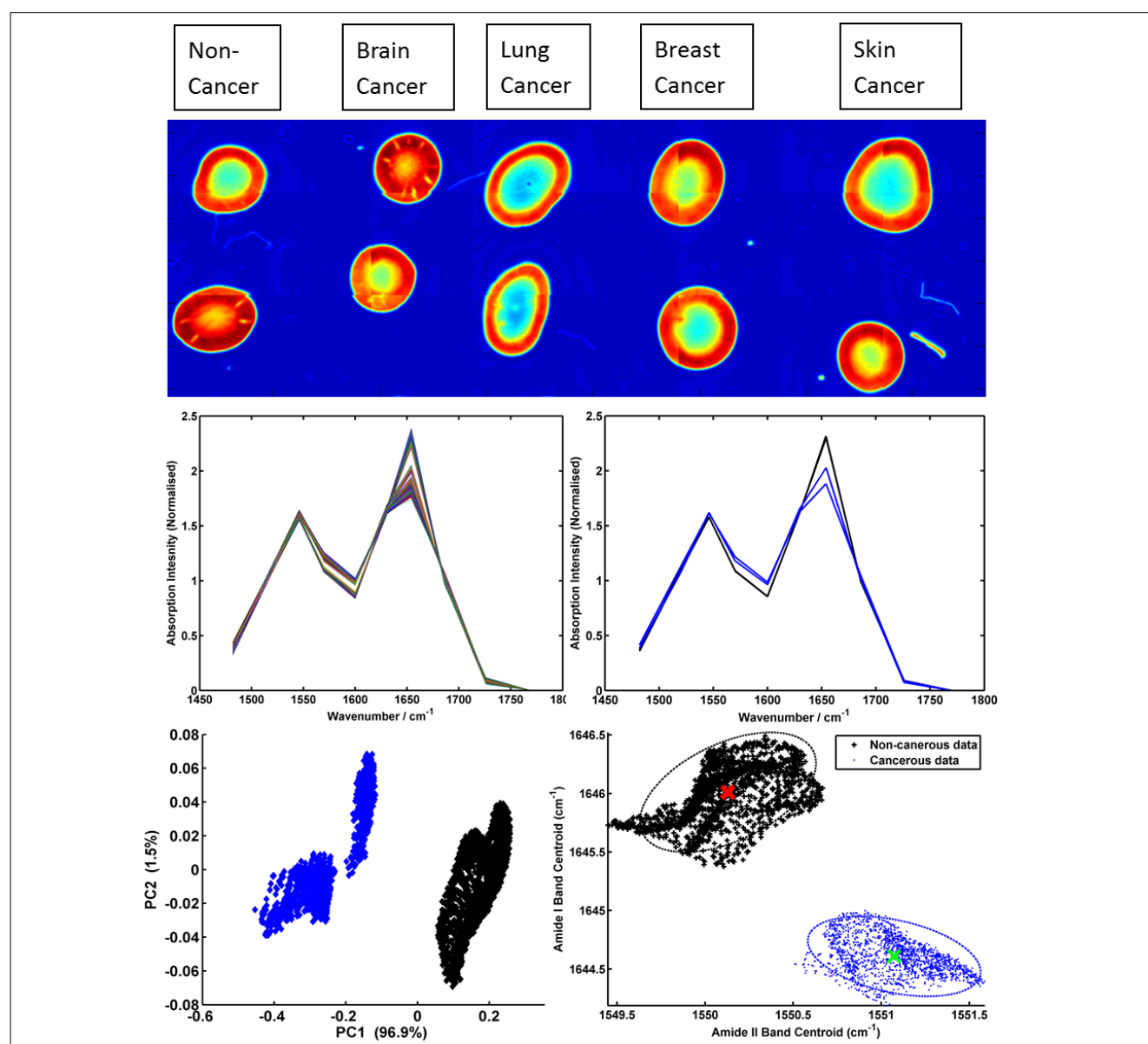
Figure 2. (A) Mosaic image of serum spots acquired using 14 discrete frequencies from non-cancer, brain cancer, lung cancer, breast cancer and skin cancer patients; (B) baseline-corrected and vector normalised serum spectra extracted from the centre of the non-cancer and brain cancer serum spots; (C) mean spectra from each non-cancer (black) and brain cancer (blue) serum spot; (D) PCA scores plot of brain cancer serum spectra (blue) and non-cancer serum spectra (black) and (E) peak centroid distribution plot of the Amide I and Amide II bands for the brain cancer (blue) and non-cancer (black) serum spectra.
