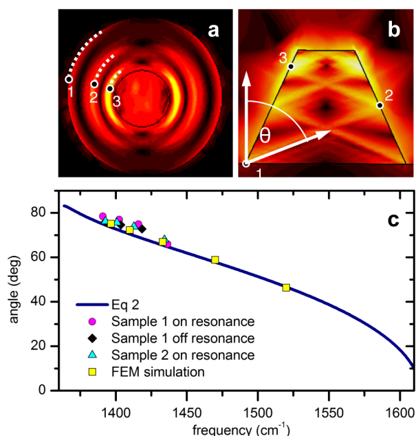
Figure 4. Polariton trajectories. (a) Numerically calculated distribution of tangential electric field at the surface of the nanocone (top view). The calculation was done for {}^U\text{TM}_{13} resonant frequency. The numbered dots and arcs indicate the radial positions of the “hot” rings observed in Figure 3. (b) The same tangential electric field distribution for the {}^U\text{TM}_{13} in the x - z cross section of the nanocone. The hot rings arise at the sidewall reflection points of the HPhP trajectories launched at the nanocone base. (c) HPhP propagation angle \theta as a function of frequency. The solid line is given by eq 2, while the symbols represent the values extracted from the near-field images (such as those in Figure 3) for the two samples, both on and off the resonance, as well as those extracted from numerical simulations.
